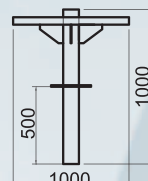
Držák K3-1.0-1.0 (M1ak, M2ak)
